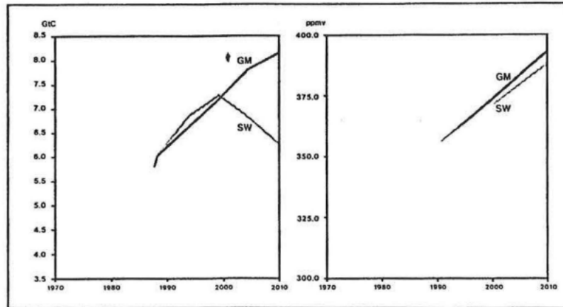
Chart 15: Global Fossil Fuel CO 2 Production to 2010
