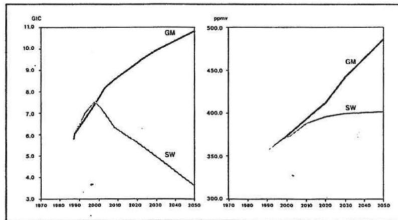
Chart 16: Global CO 2 Production to 2050
