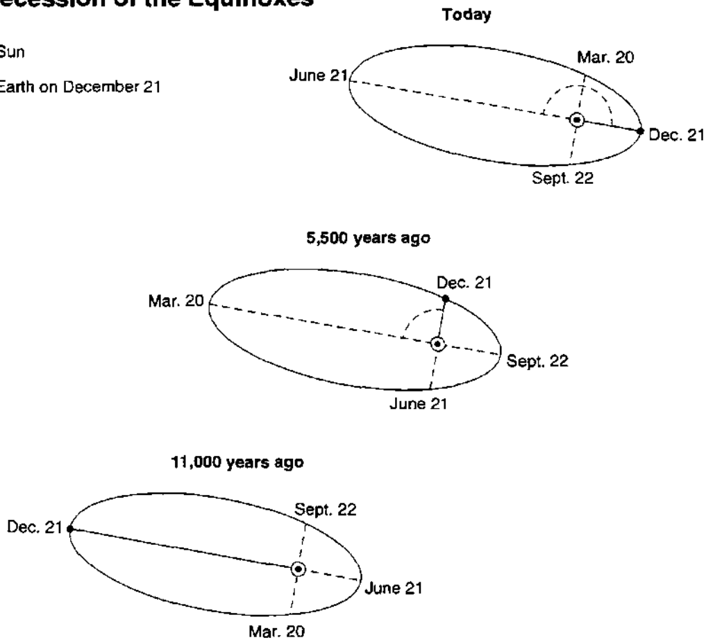
Figure 1: Schematic Illustrations of Orbital Changes of Earth (From Lindzen - 1994)
