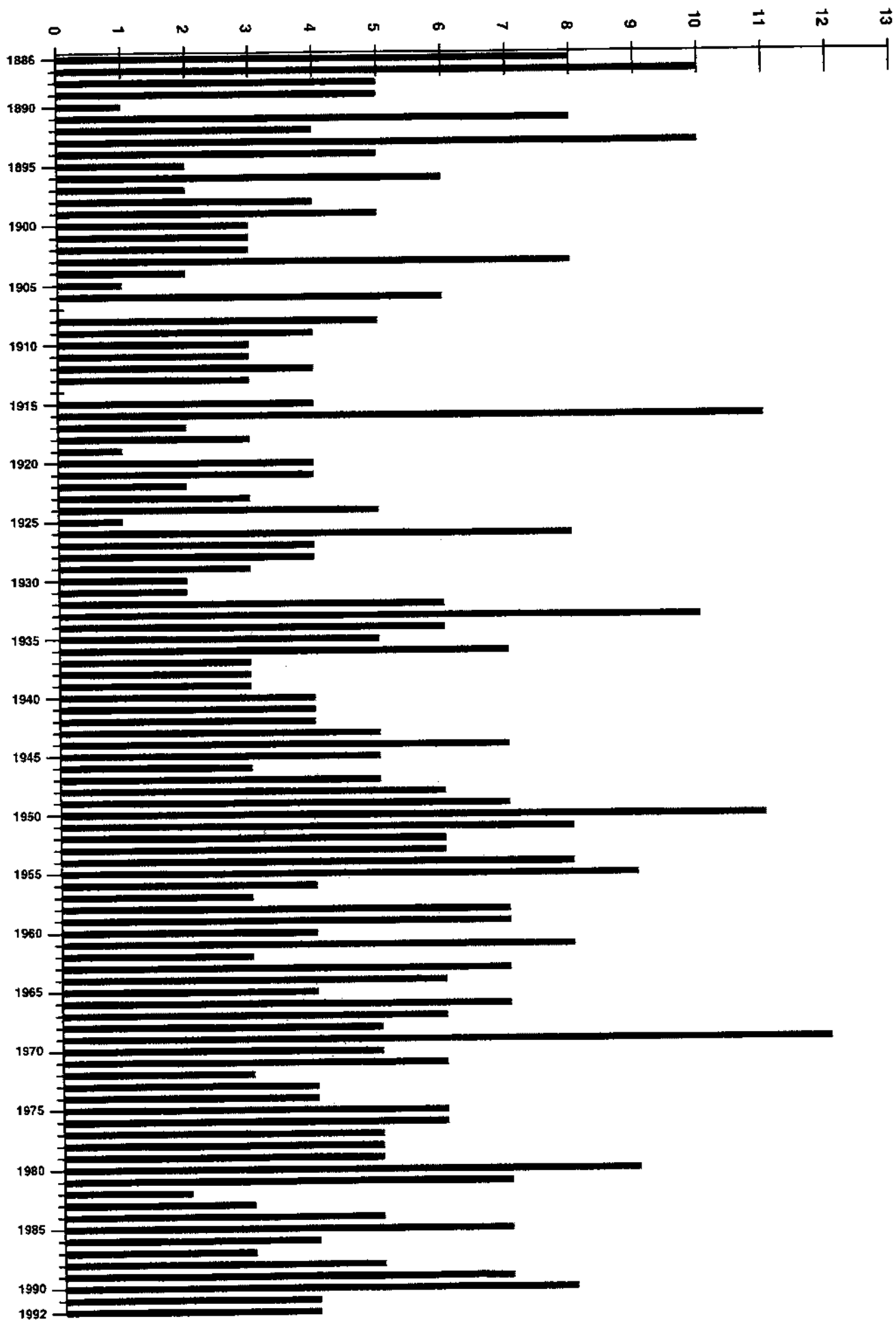
Figure 12: Number of tropical storms which eventually became hurricanes
