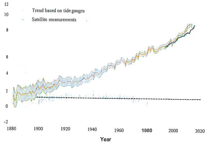
Global Average Absolute Sea Level Change, 1880-2015
